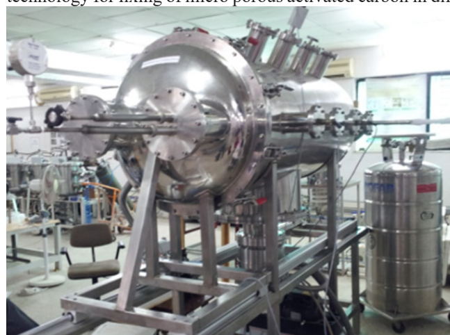
Figure A.2.3.2 Single Panel Cryopumping Facility
