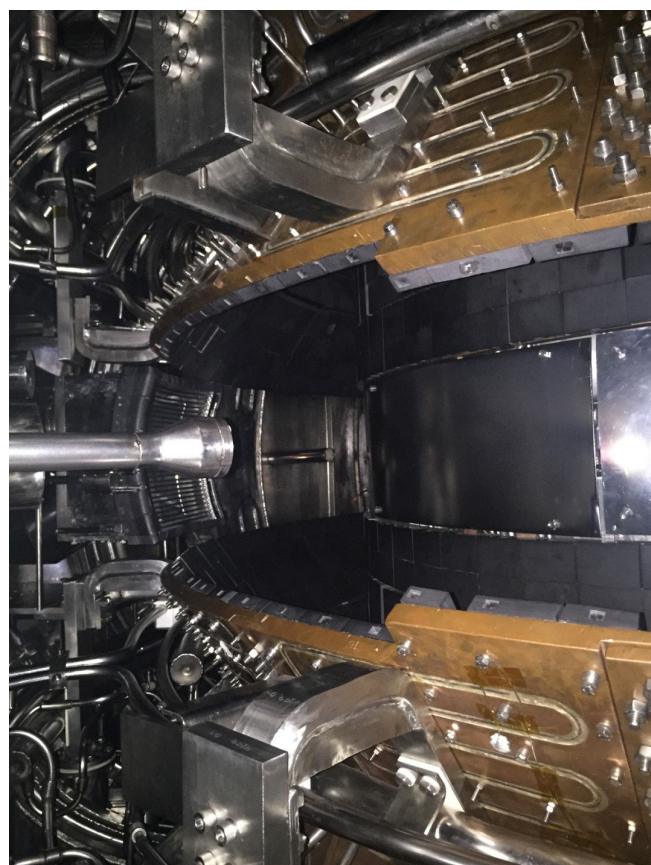
Figure A.1.2.3 SST-1 up-gradation is going on with plasma facing components
