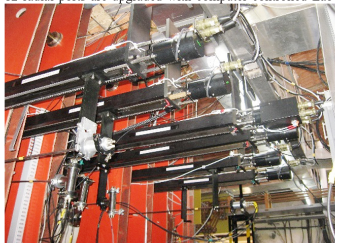
Figure A.3.1.3 A few large, linear motion, vacuum interfaced probe drives with \sim 1\text{ m} travel length
