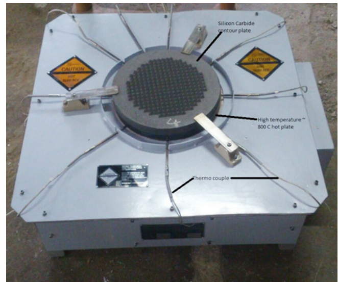
Figure B.2.9 Indigenously developed high temperature (~ 800 °C) blackbody source for calibration of 70 to 1000 GHz
