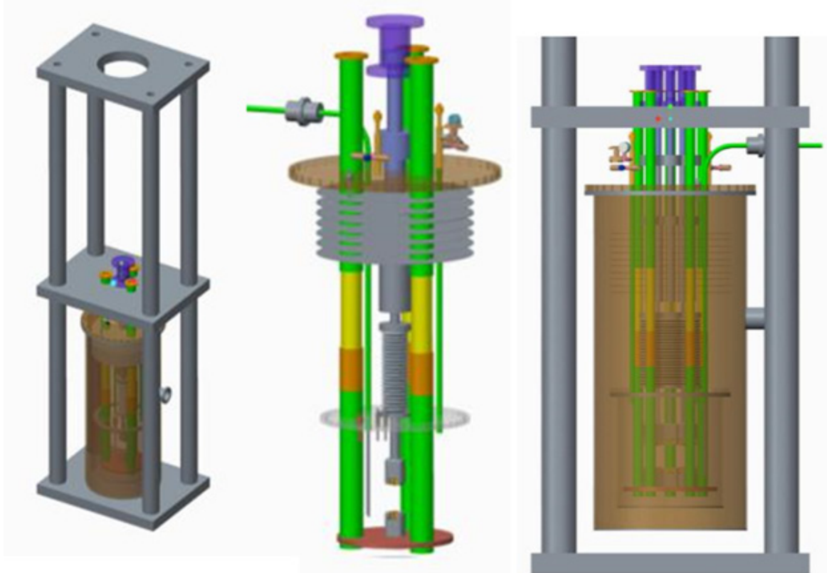
Figure A.2.1.3 . Mechanical characterization facility at low temperature
