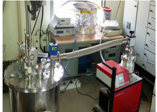
Figure A.2.1.2 Cryogen free facility (Cabling, jacketing and Winding) for manufacturing of superconducting central solenoid are under progress as shown.
