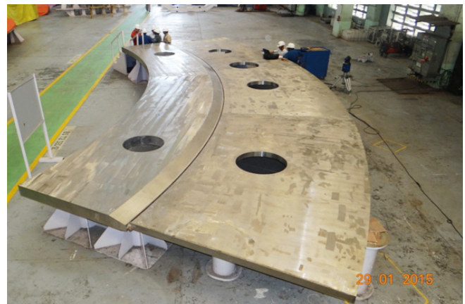
Figure B.2.2 Cryostat Base Section Tier -2 – fabrication in advanced stage
