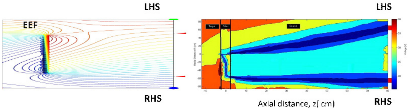
Figure A.3.1.1 Correlation of peak floating potential profile in source, Electron Energy Filter and Target region with the simulated field pattern of coupled magnetic field and ambient magnetic field of LVPD
