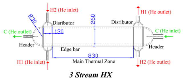
3 Stream HX Figure A.2.5.1 Overall dimension (mm) of Prototype 3-stream heat exchanger
