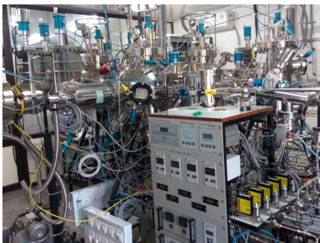
Figure B.1.5 Multi chamber multi magnetron (MCMM) vacuum system installed
