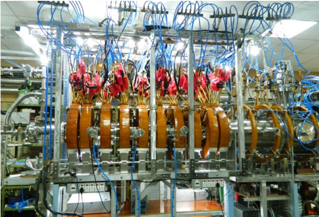
Figure A.3.6.1 Picture of Inverse Mirror Plasma Experimental Device (IMPED) set up at basic plasma laboratory
