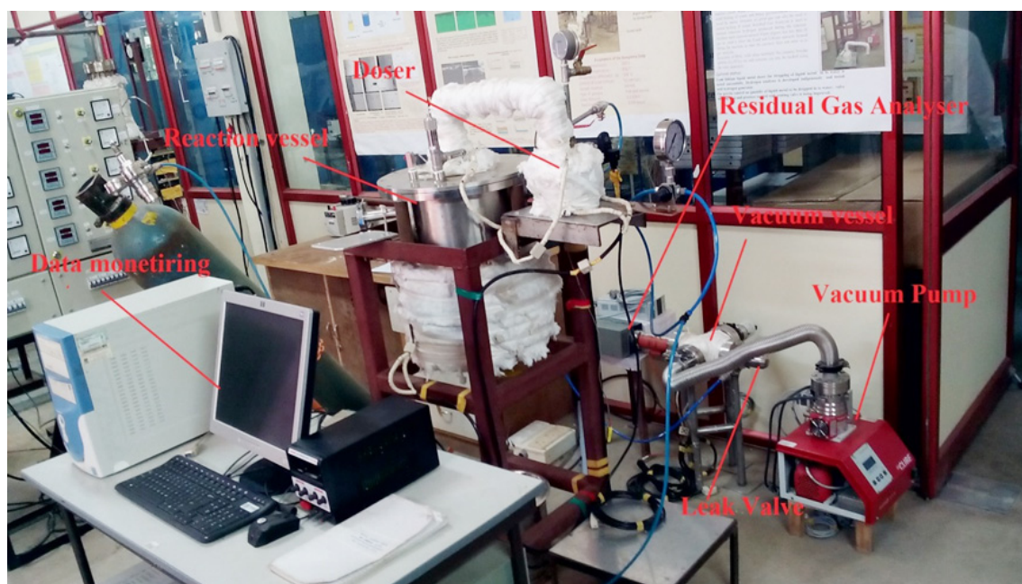
Figure A.2.4.2 Lead-Lithium- water safety experiment set up
